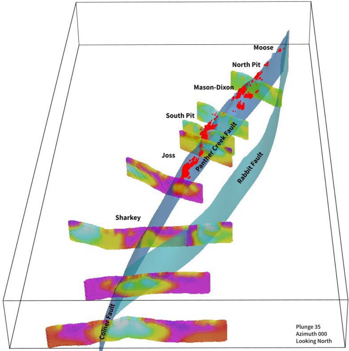
Figure 2: Perspective View of Reprocessed CSAMT Resistivity Showing Key Structures 2023 Mineral Resource Blocks > 2 g/t Au
