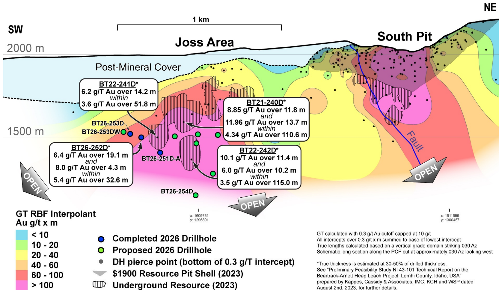
Figure 2: Long Section – South Pit to Joss Area (Looking West)
